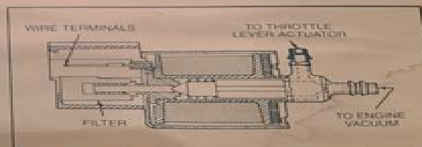
Figure 7-5. Throttle Return Control Solenoid Vacuum Control Valve
