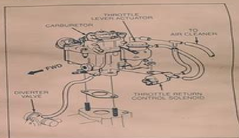
Figure 7-4. Throttle Return Control Solenoid Valve Location (4.8L Gasoline Engine)
