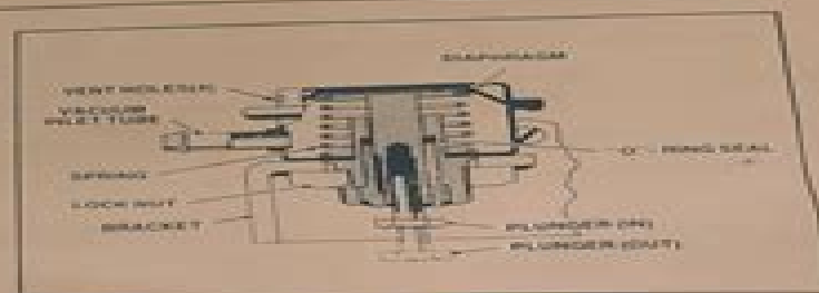
Figure 7-3. Throttle Lever Actuator (4.8L and 5.7L Gasoline Engines)
