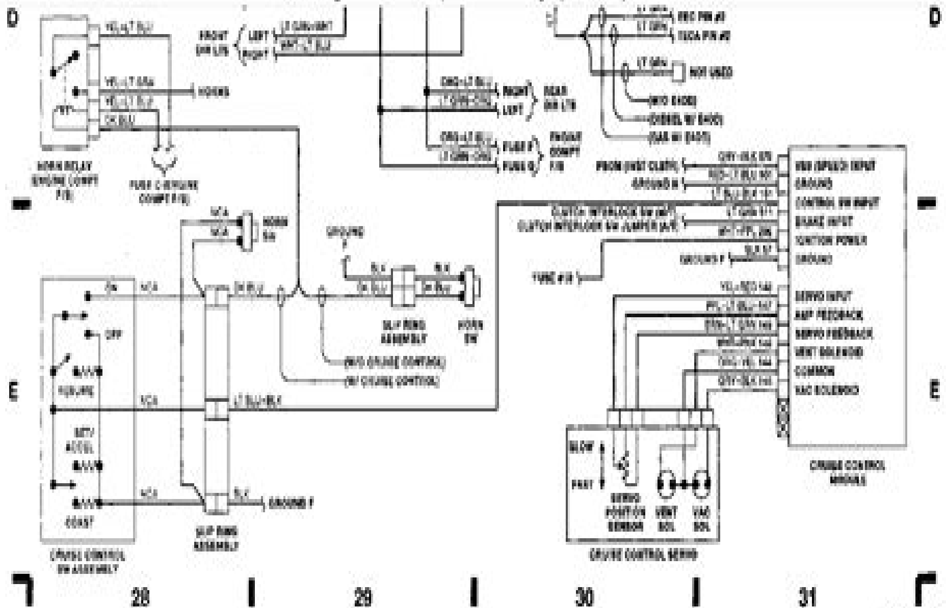
Fig. 8: Clutch Interlock, Cruise Control/Wiper (Grids 28-31)
