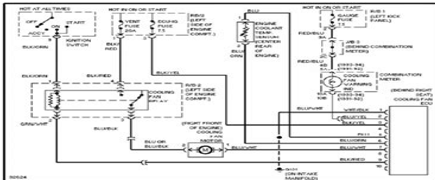
Engine Compartment Cooling Fan Circuit
