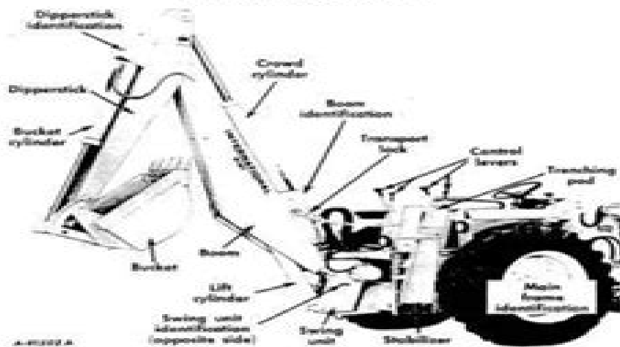
Location of units and parts. International 3721 Backhoe shown as International 3636 Loader Tractor.
