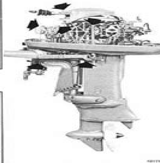
Figure 2-2. Port Side, 40 H.P. Manual Start
