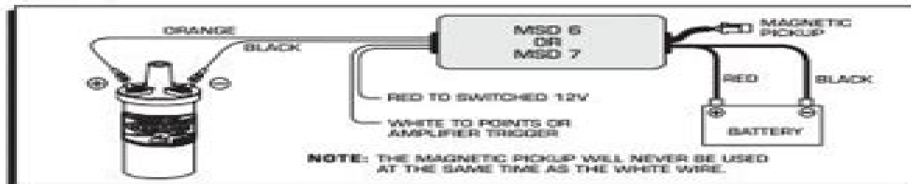
Figure 1 Wiring to an MSD 6 or 7 Series Ignition Control.
