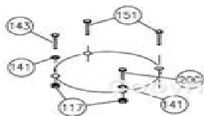
HONDA ENGINE MOUNTING
