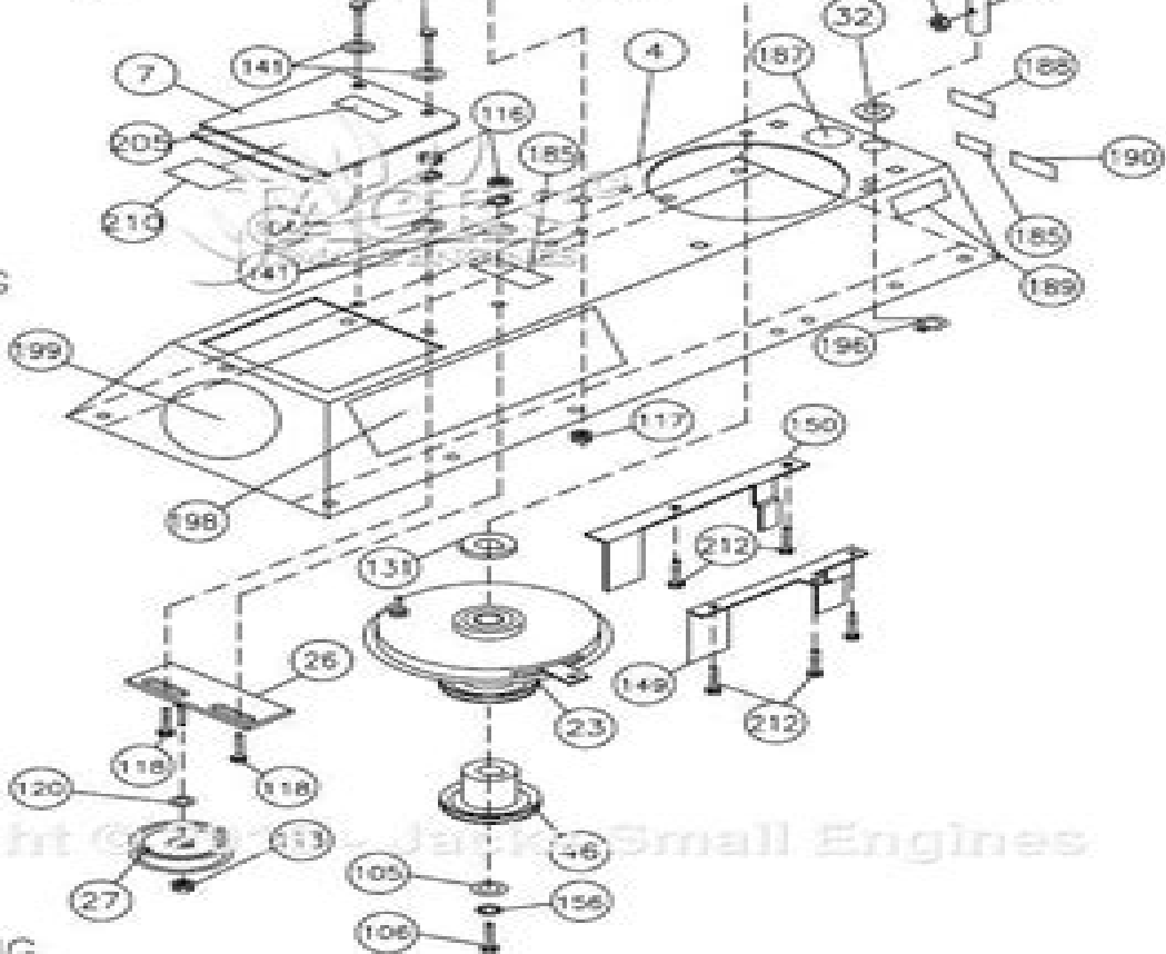
HEB ENGINE MOUNTING
