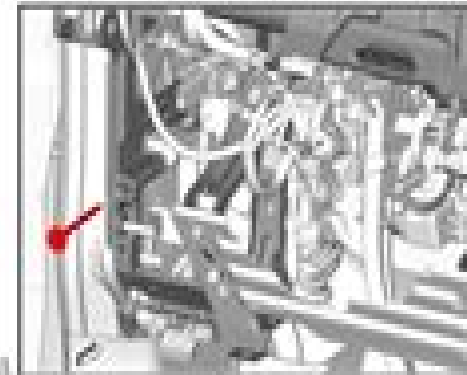
Instrument Panel Tie Bar Bolt (1) - Install and tighten 9 N.m (66 lb in)
