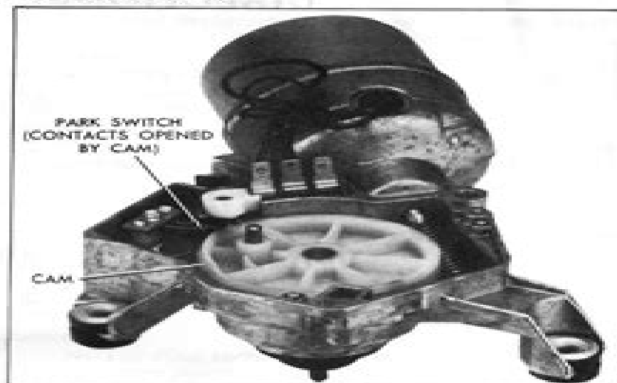
Fig. 17—Gear in PARK Position—Contacts Open
