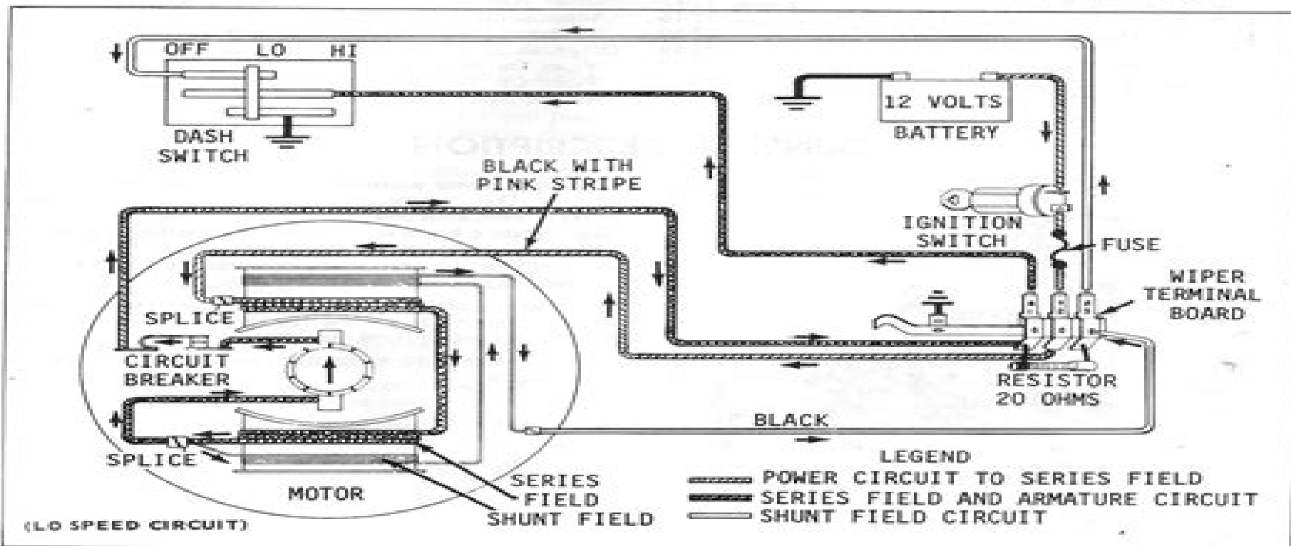
Fig. 18—LO Speed Circuit
