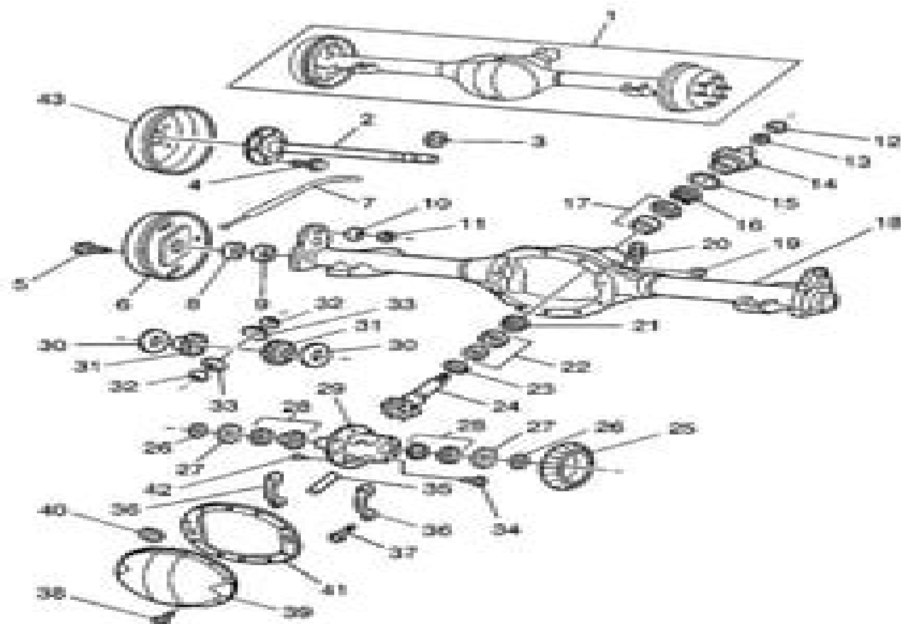
Fig. 1: Rear Drive Axle Disassembled View Courtesy of GENERAL MOTORS CORP.
