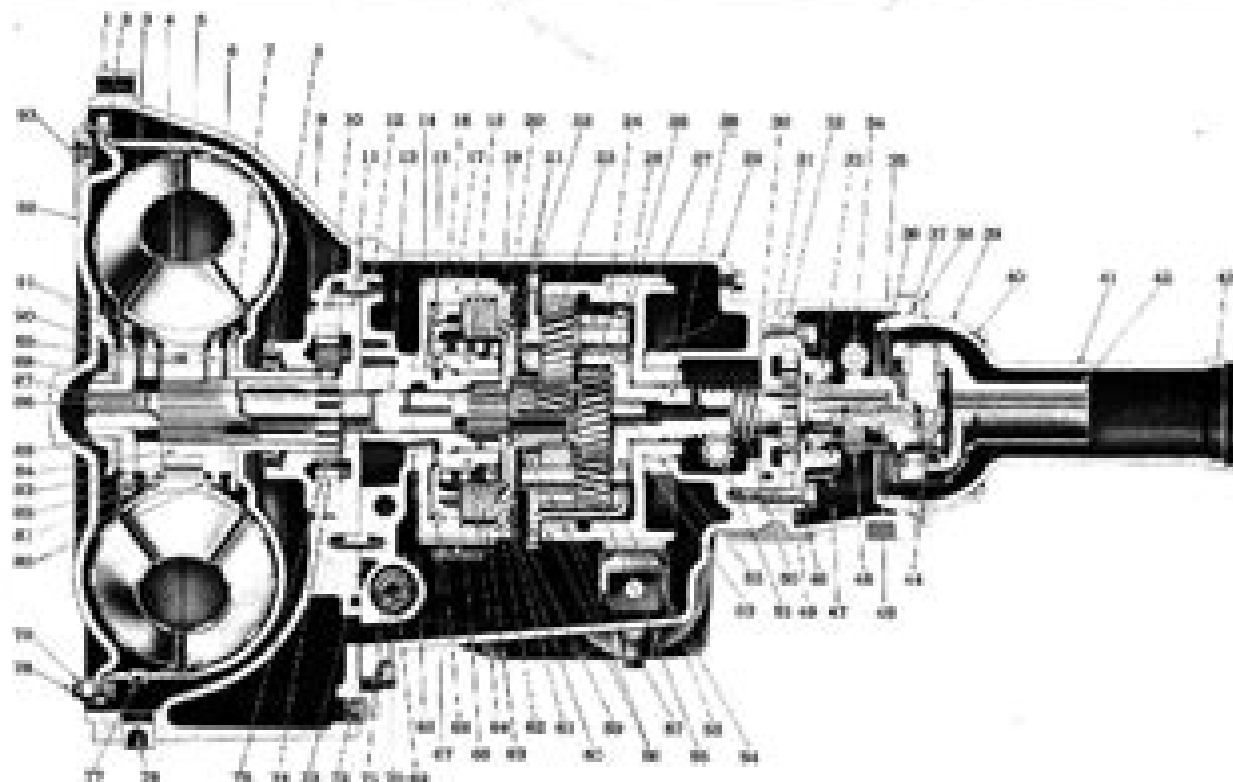
Fig. 181—Transmission Cross Section
