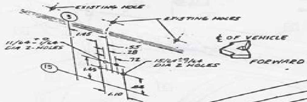
VIEW B V-8 ENG. R.H. SIDE
