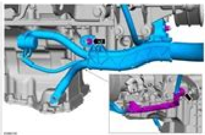
11. Disconnect the coolant hoses. (Disconnect the retainers and remove the coolant hoses.)
