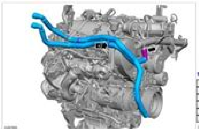
11. Disconnect the coolant hoses. (Disconnect the retainers and remove the coolant hoses.)
