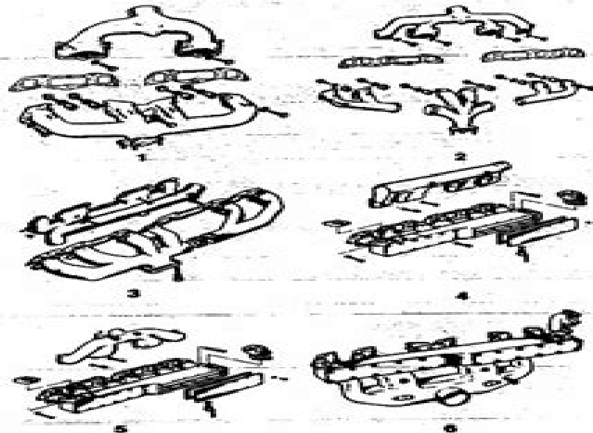
Fig. 2 A selection of manifolds used with 2700 Range Engines.
