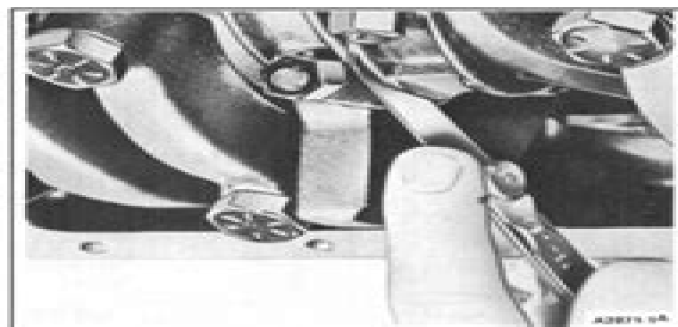
FIG. 44 Checking Connecting Rod Side Clearance
