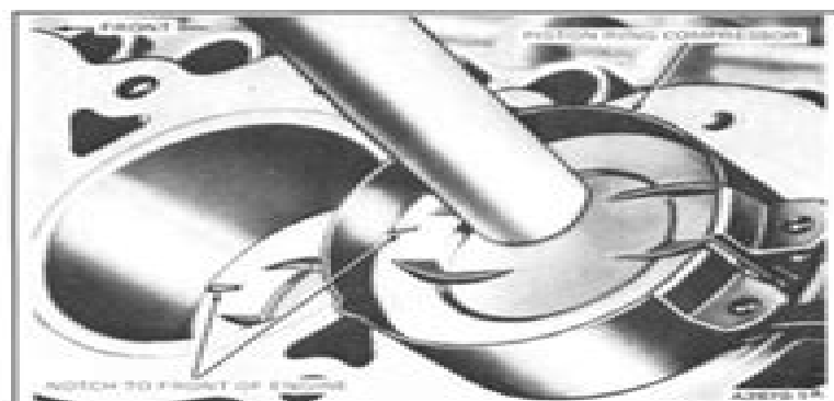
FIG. 43 Installing Piston
