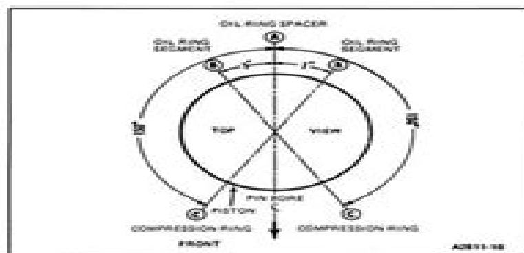
FIG. 42 Piston Ring Spacing
