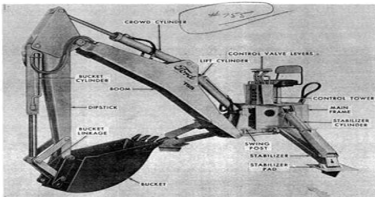
Figure 1 Series 753 Backhoe
