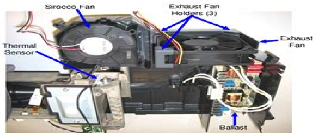
Figure 3: Lower Duct (Top View)
