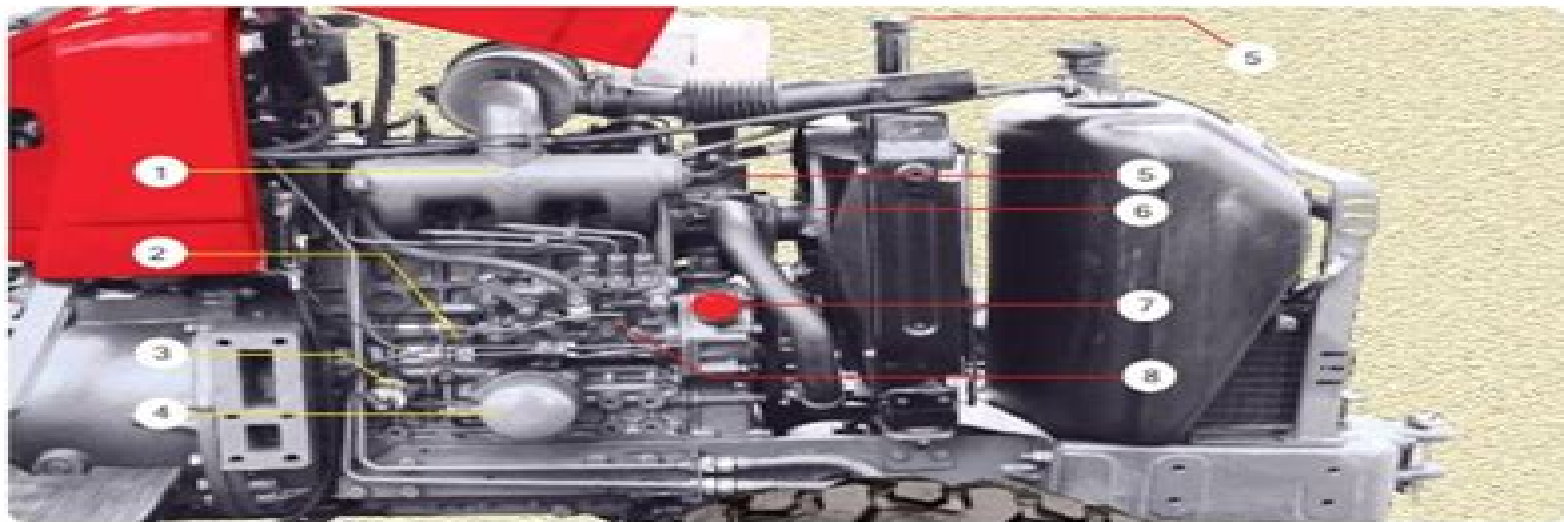
L.H View : 1. Intake Manifold. 2. Dipstick Engine 3. Oil Pressure Switch 4. Oil Filter Engine. 5. Thermostat. 6. Fan Belt 7. Oil Filler Cap. 8. Fuel Injection Pump
