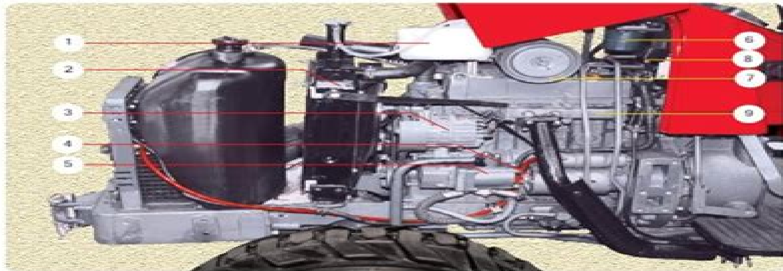
R.H View : 1. Expansion Tank. 2. Radiator. 3. Alternator 4. Starter Motor 5. Hydraulic Pump 6. Fuel Filter 7. Air Cleaner 8. Fuse box 9. Exhaust Manifold.
