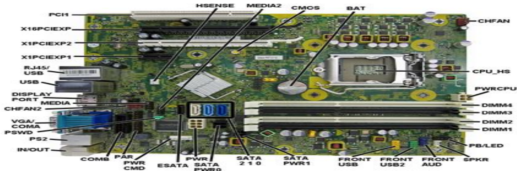
System Board Connectors and Jumpers (component location may vary)
