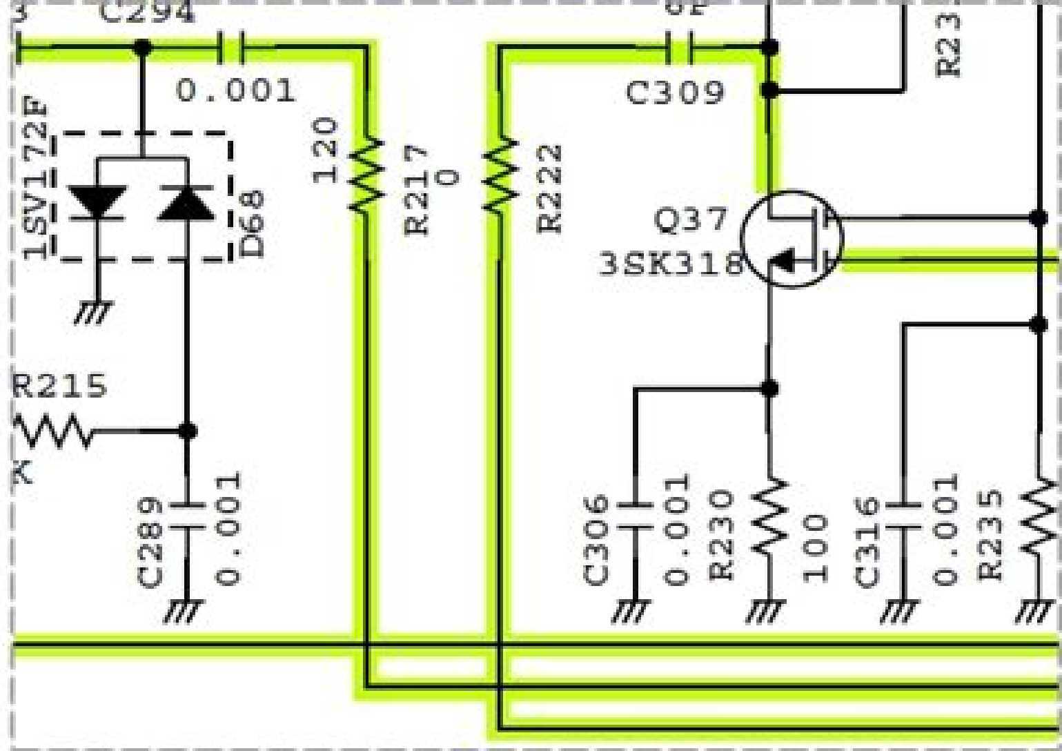
Preview: ICOM IC-2820H schematic diagram
