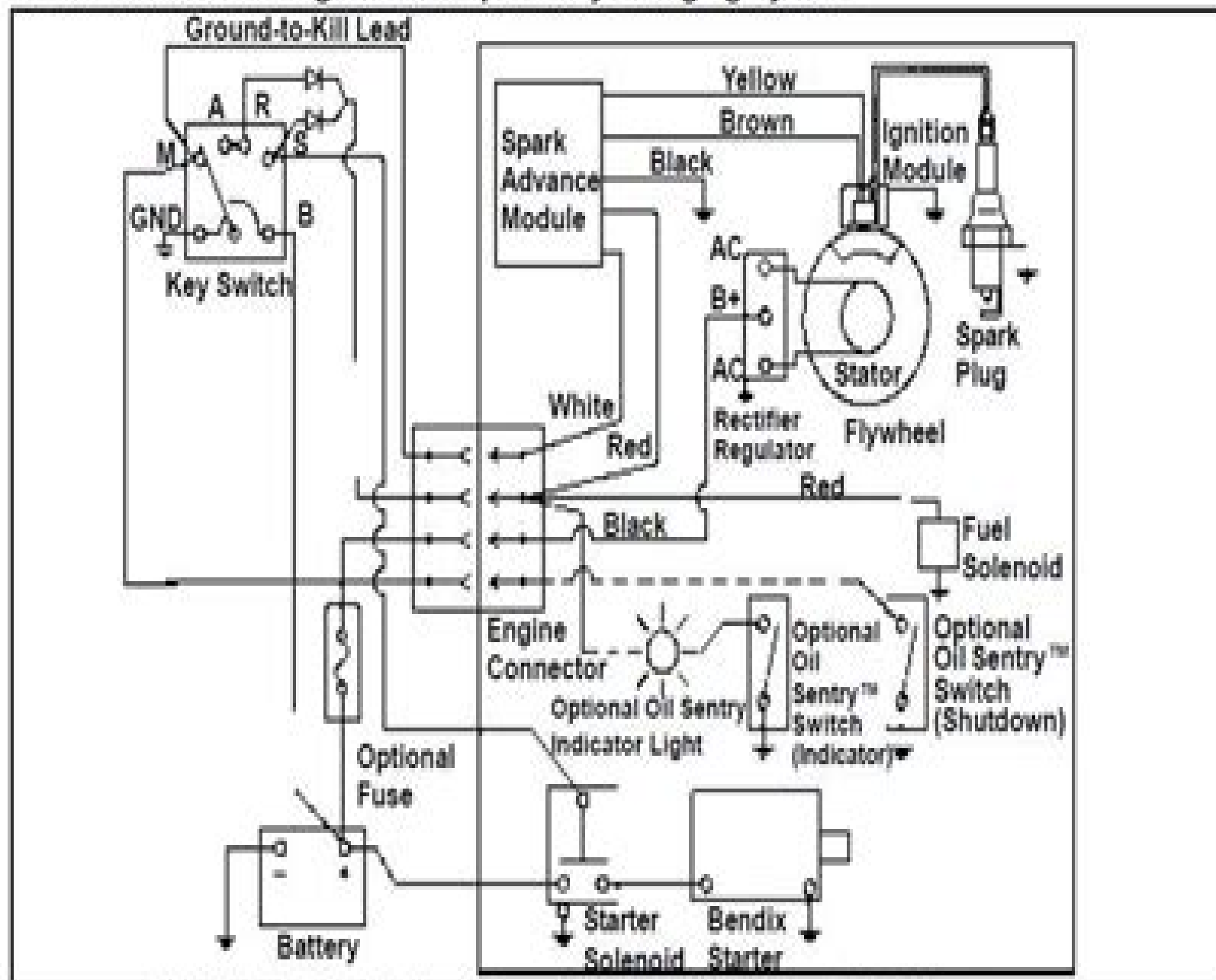
CV16 Electric Start Engines/15 amp Regulated Battery Charging System.
