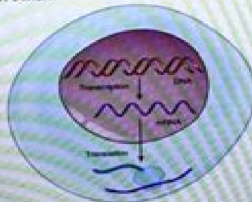
Figure 4. Transcription-translation summary.
