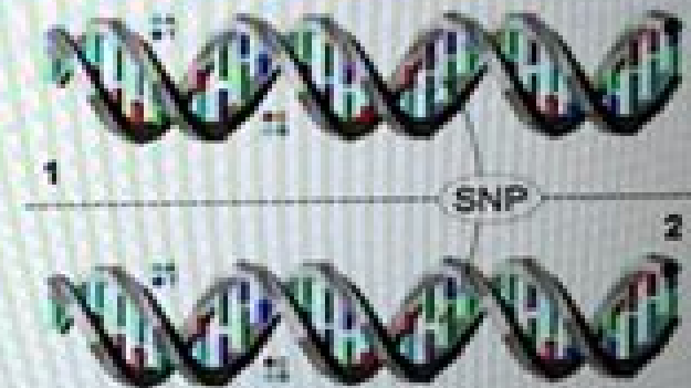
Figure 3. SNP.
