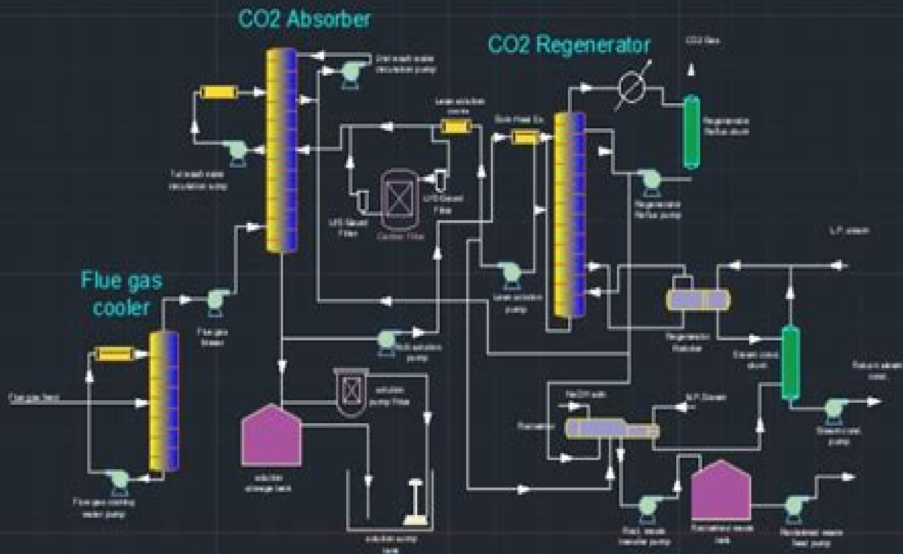
Process Flow Diagram (PFD) for CO2 Recovery Plant
