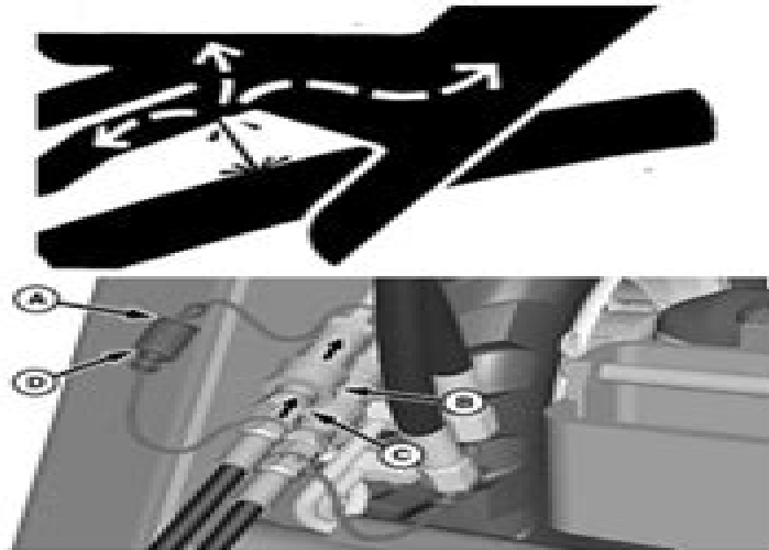
A—Plug (1 per female coupler) C—Coupler, Male (1 per connection) B—Coupler, Female (1 per connection) D—Cap (1 per male coupler)
