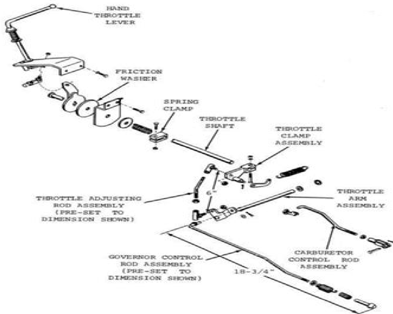
Fig. 3 — Parts Book View of MF 125 Gas Tractor Throttle Linkage
