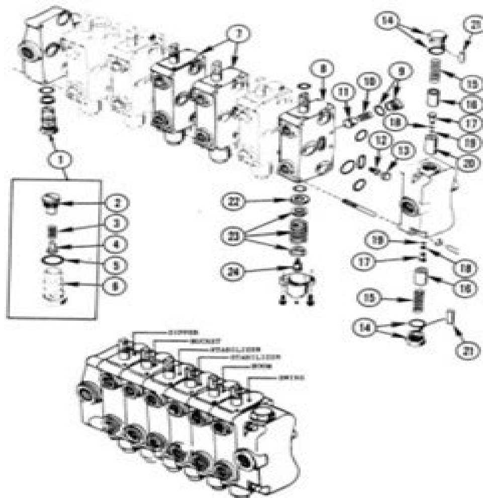
Fig. 14 — End Plates, Swing and Stabilizers Sections of Control Valve
