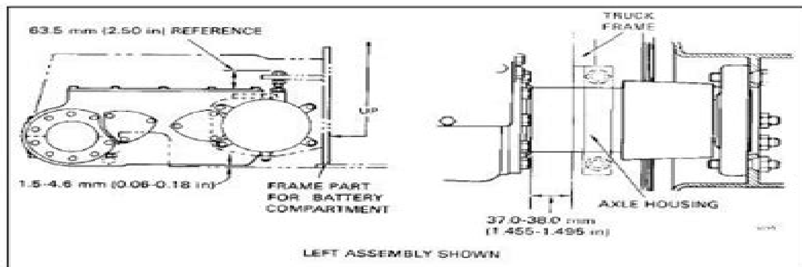
FIGURE 4. TRANSAXLE ALIGNMENT
