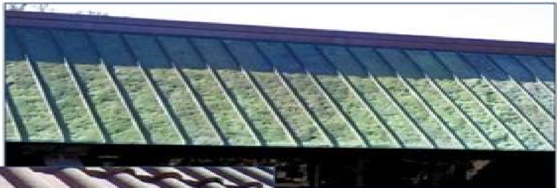
Photo 5 – Damage to copper standing seam.
