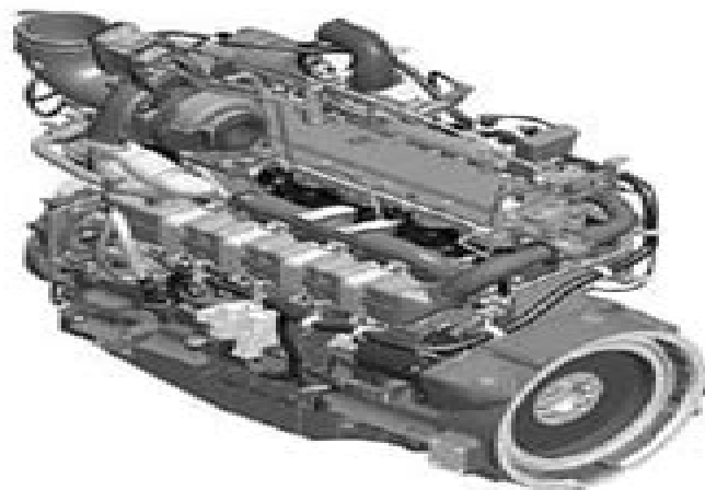
3/4 left rear view—6055HFC63 Engine
