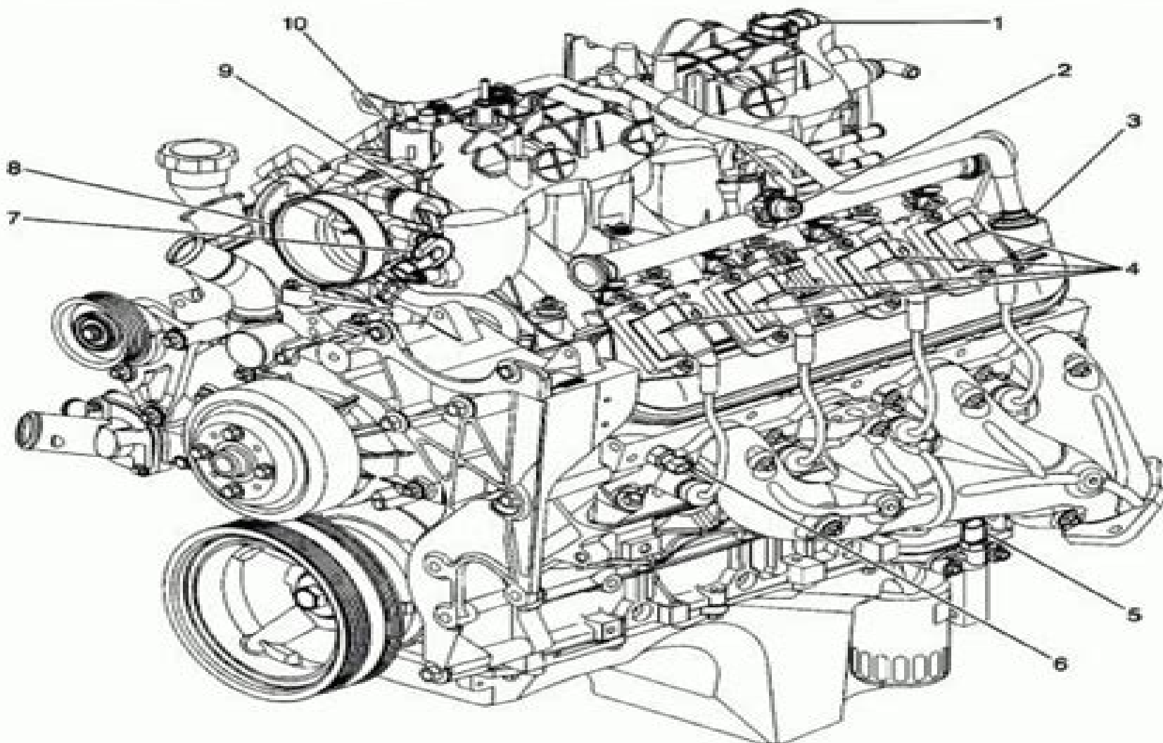
Full Engine View Left Side (4.8L, 5.3L, 6.0L)
