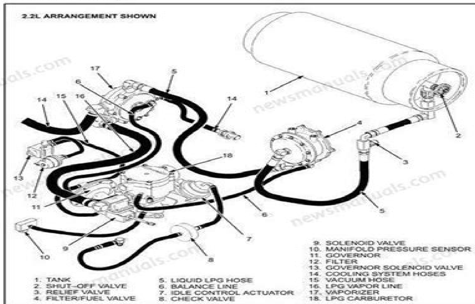
FIGURE 1. ARRANGEMENT FOR GM 2.2L ENGINE
