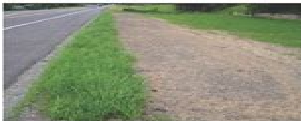
Media Filter Drain Along SR 14 in Clark County, WA. Source: Washington State DOT, 2011.
