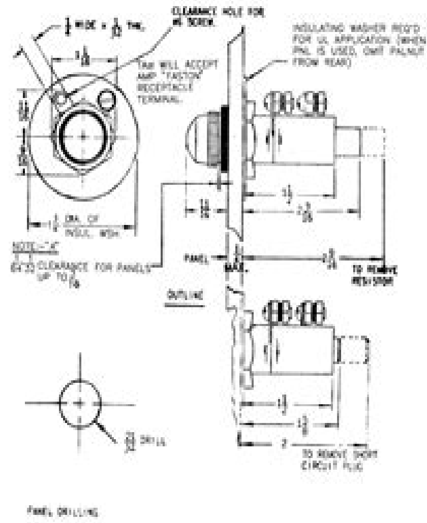
Figure 4 INSTALLATION, OUTLINE AND PANEL DRILLING FOR RECESSED INDICATING LAMP TYPE ET-12
