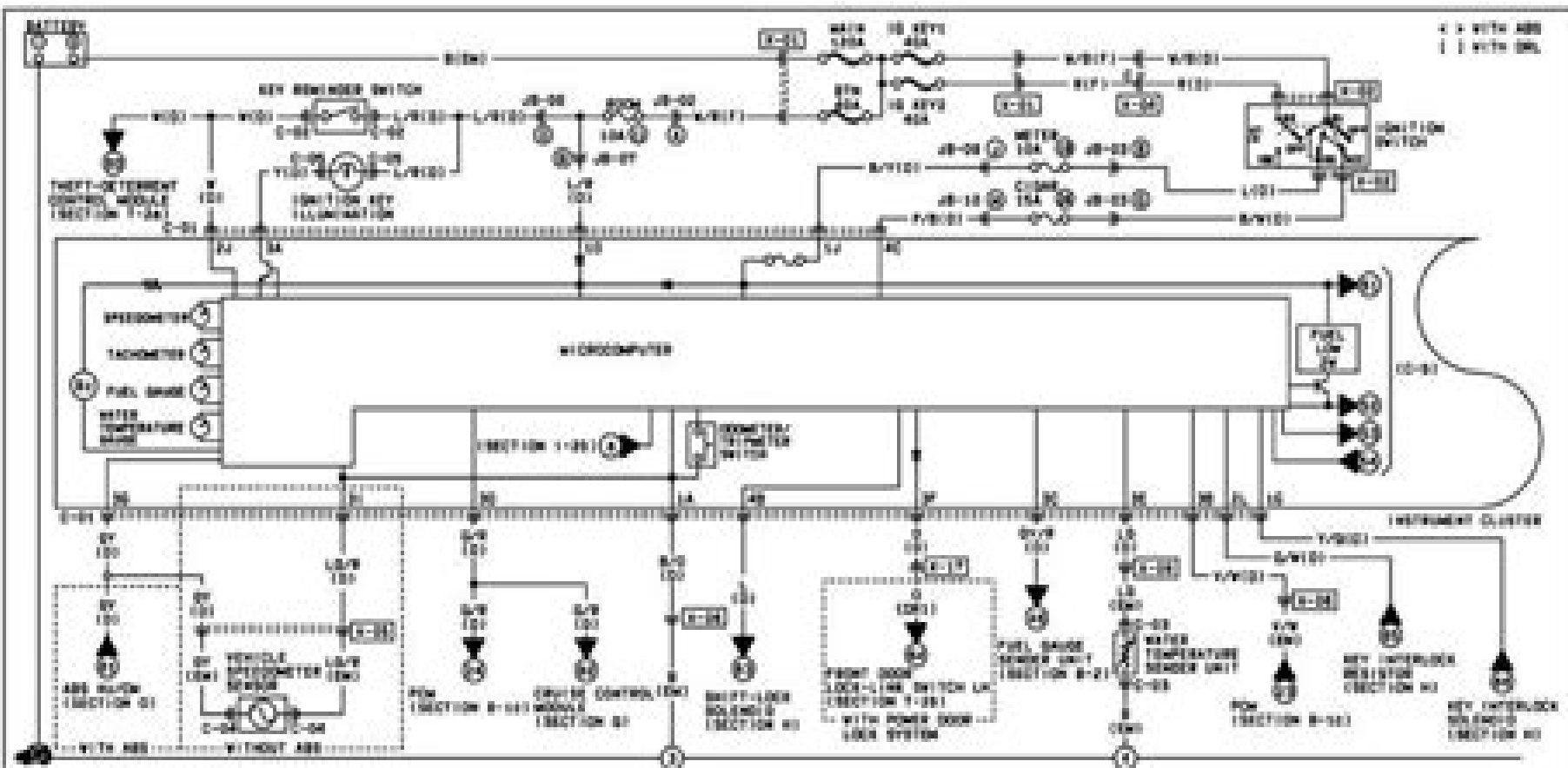
C-01 INSTRUMENT CLUSTER (2)
