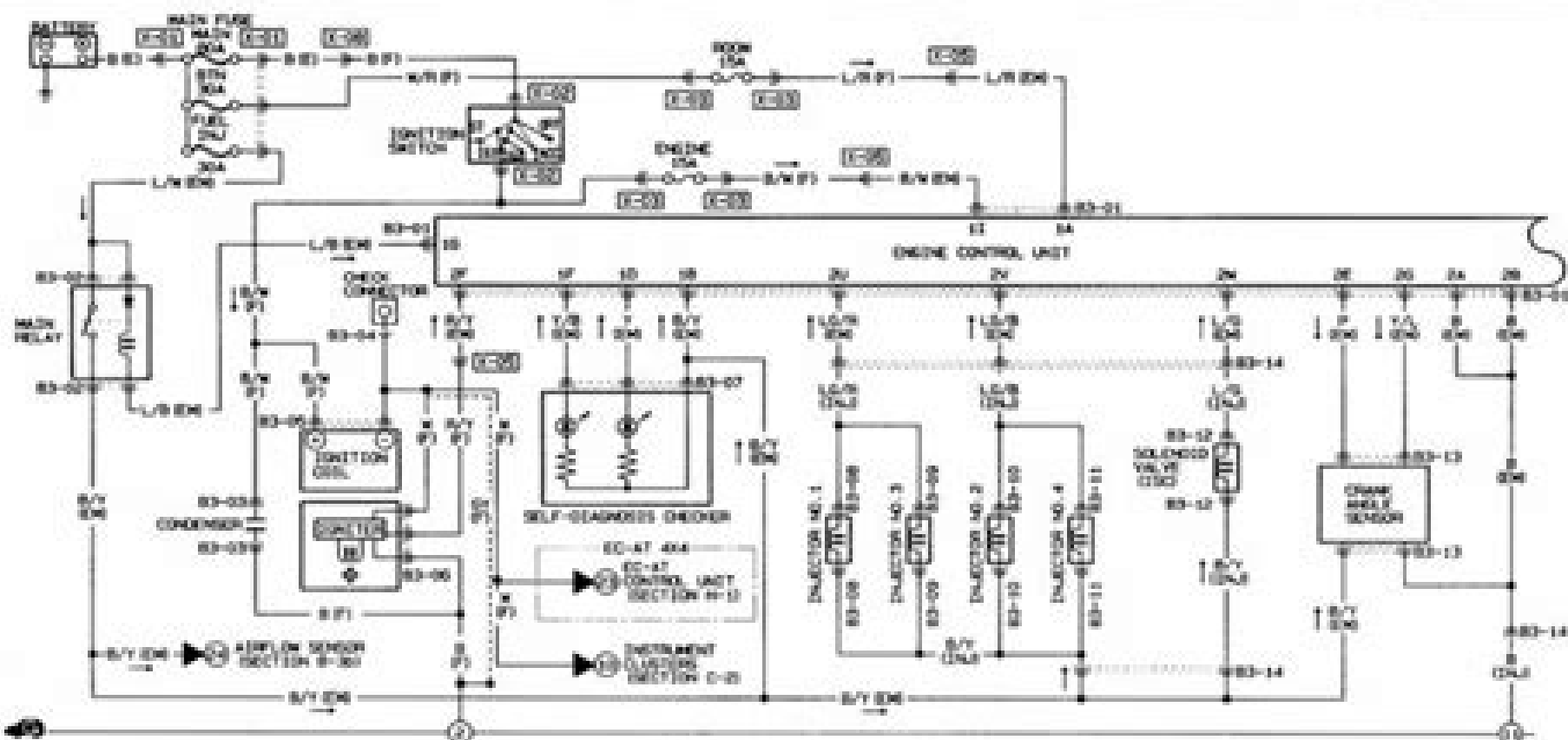
B3-31 ENGINE CONTROL UNIT (EM)
