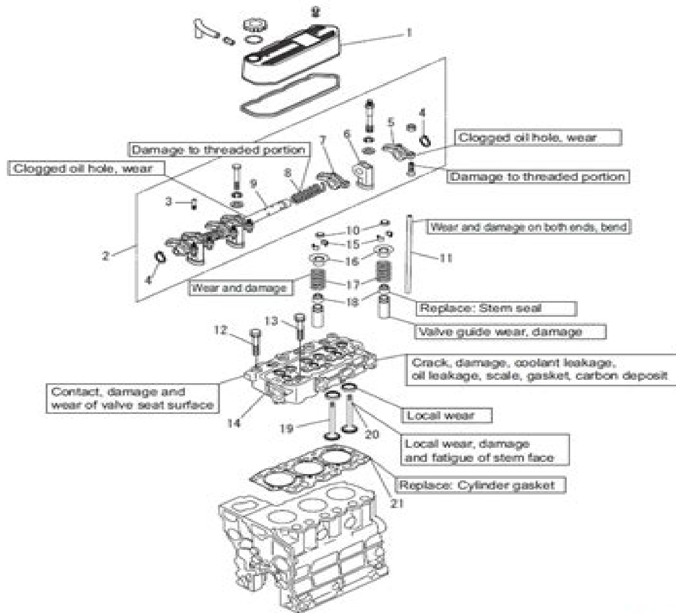
Disassembling and inspecting cylinder head and valve mechanism
