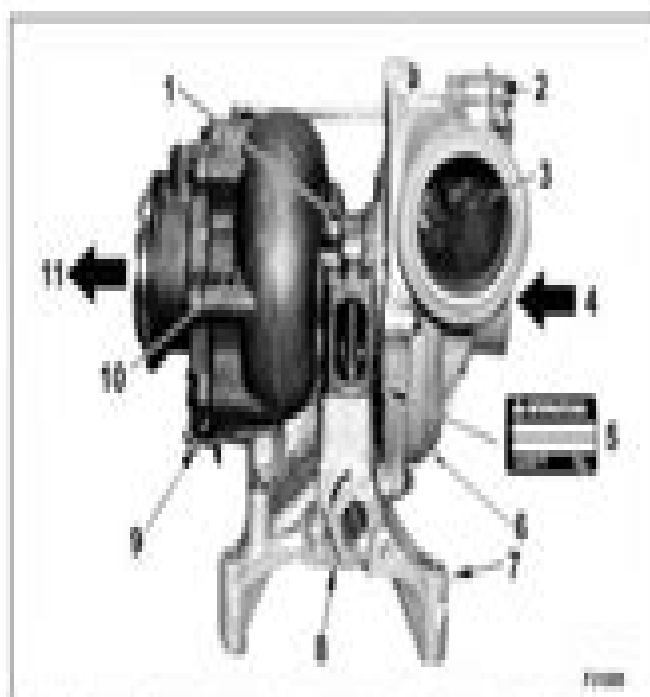
Figure 20 Garrett Turbocharger (Garrett L60) Through 200 Model Year (200-25 Model Years)
