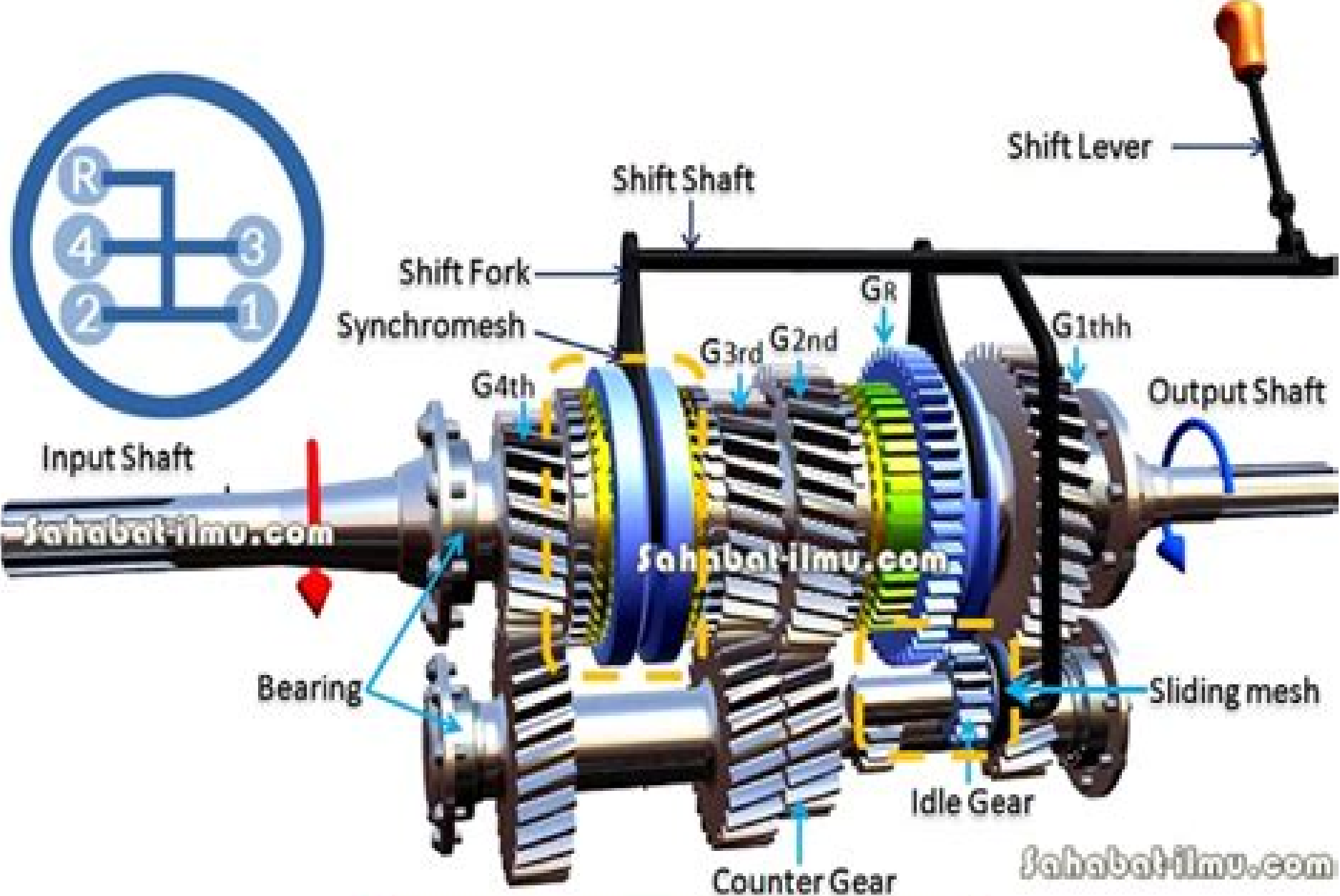
Manual Transmission
