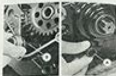
A. Shift Shaft Oil Seal Guide, 57001-204 B. External Shift Mechanism
