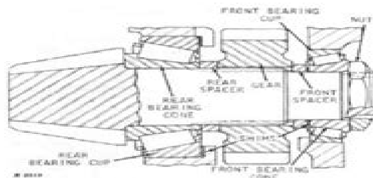
Fig. 130-20-67—Differential Bevel Pinion Shaft
