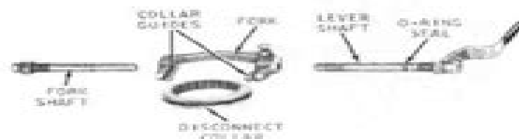
Fig. 130-20-65—Tow Disconnect Parts
