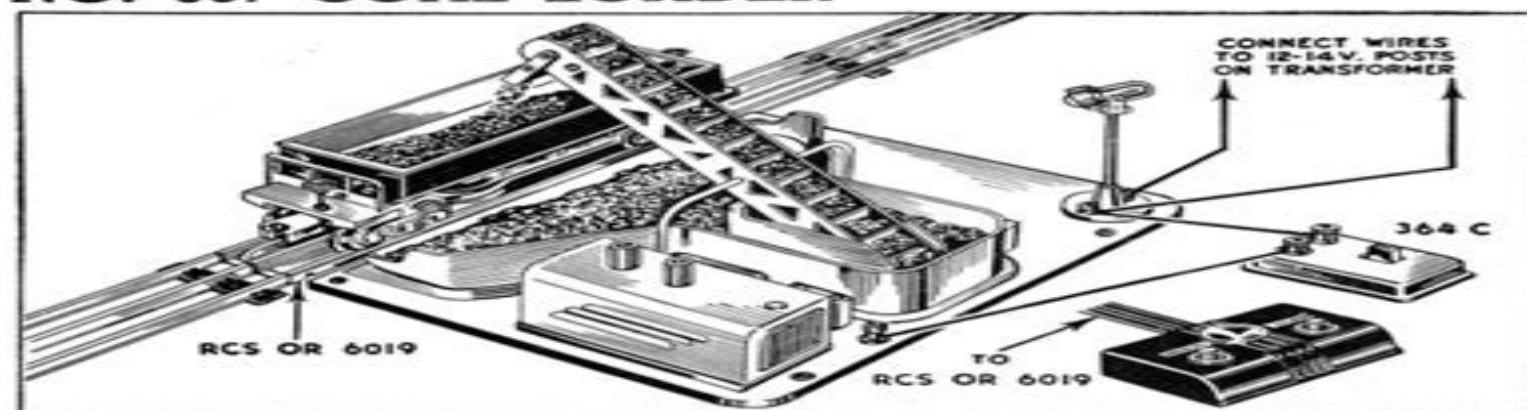
Figure 36—Coal Loader Layout
