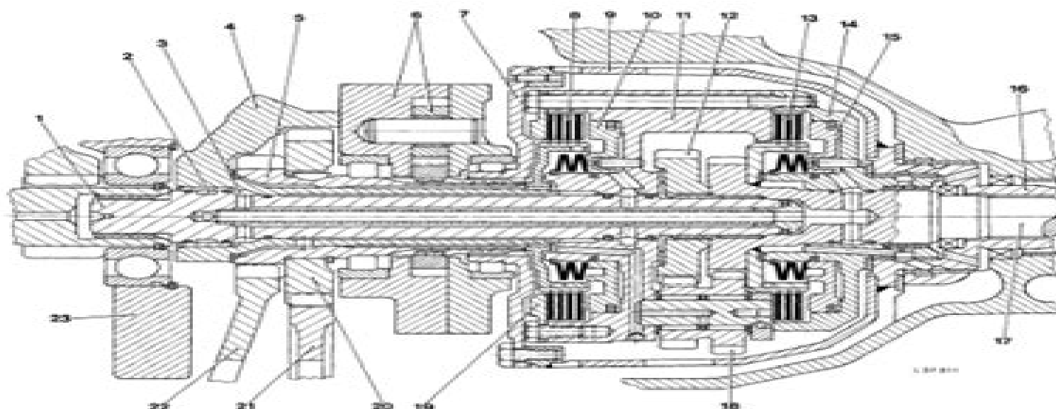
Fig. 1 — HIGH-LOW Shift Assembly, Sectional View
