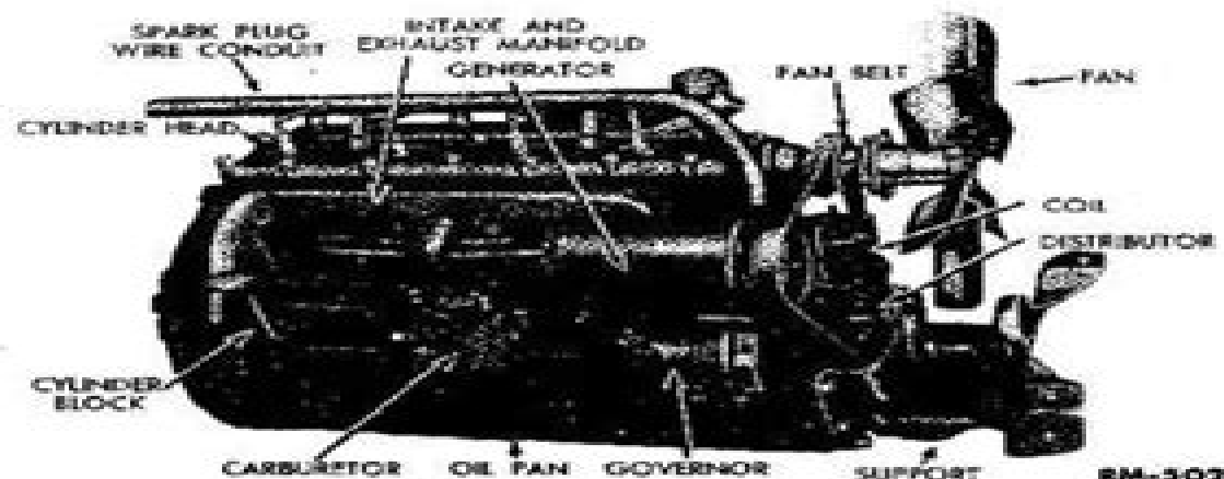
Fig. 2—Right 3/4 Front View of Engine
