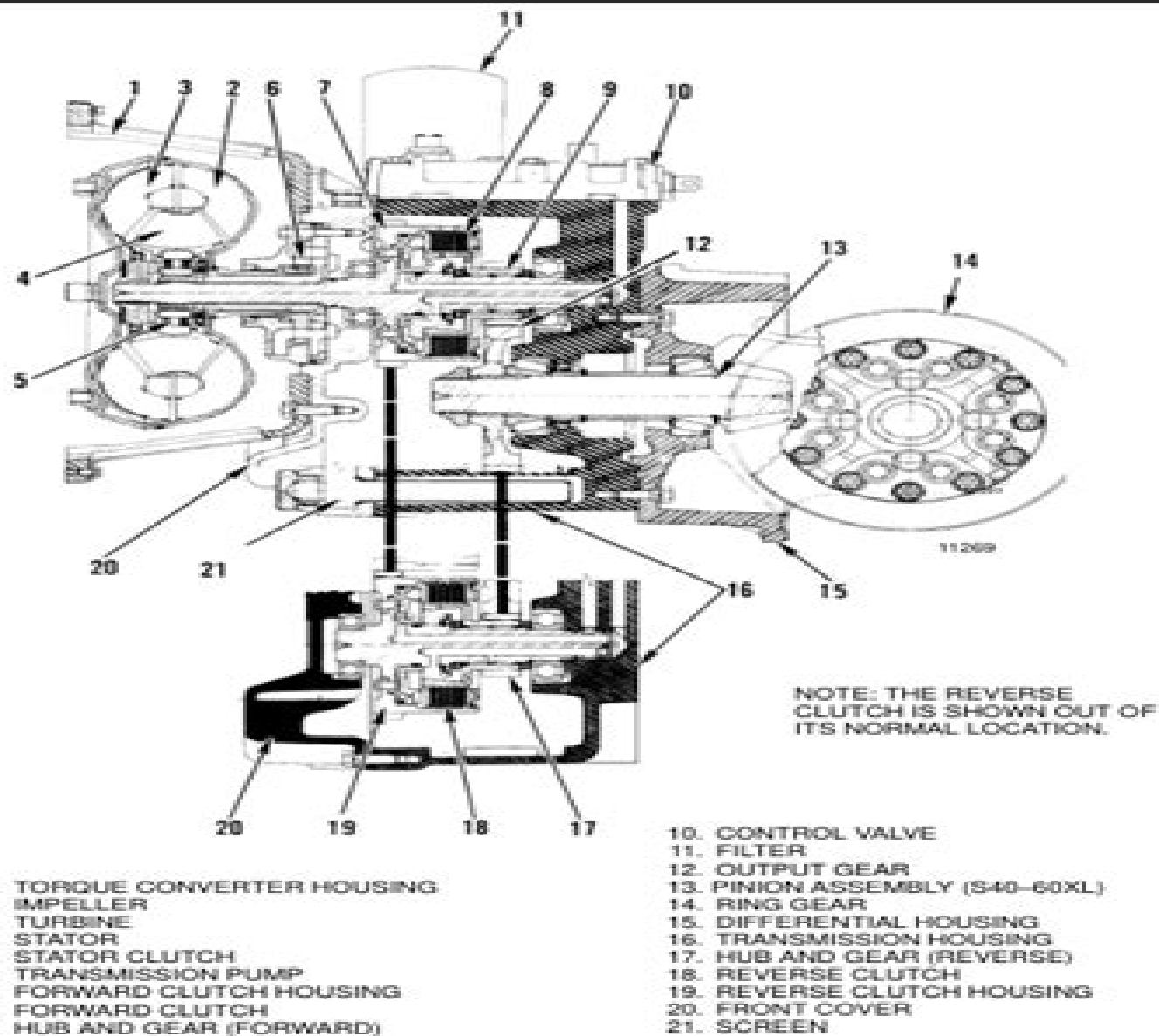
FIGURE 6. TRANSMISSION, SECTION VIEW
