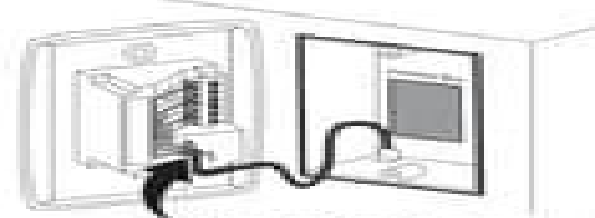
Mounting Detector/Wire Support Loop
