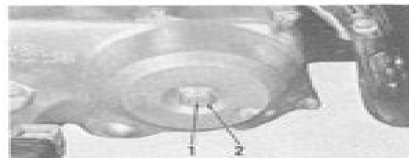
Fig. 4—Adjust clutch action on automatic clutch by loosening nut (2) and turning adjusting screw (1) as outlined in text.
