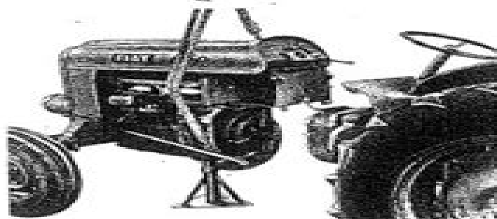
Fig. 83. - Removal of engine, with front axle.
