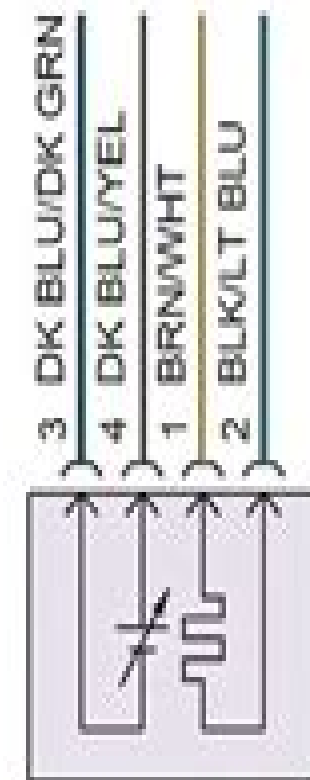
OXYGEN SENSOR 1/2 (A/T: BELOW TRANSMISSION, IN LEFT EXHAUST PIPE)
