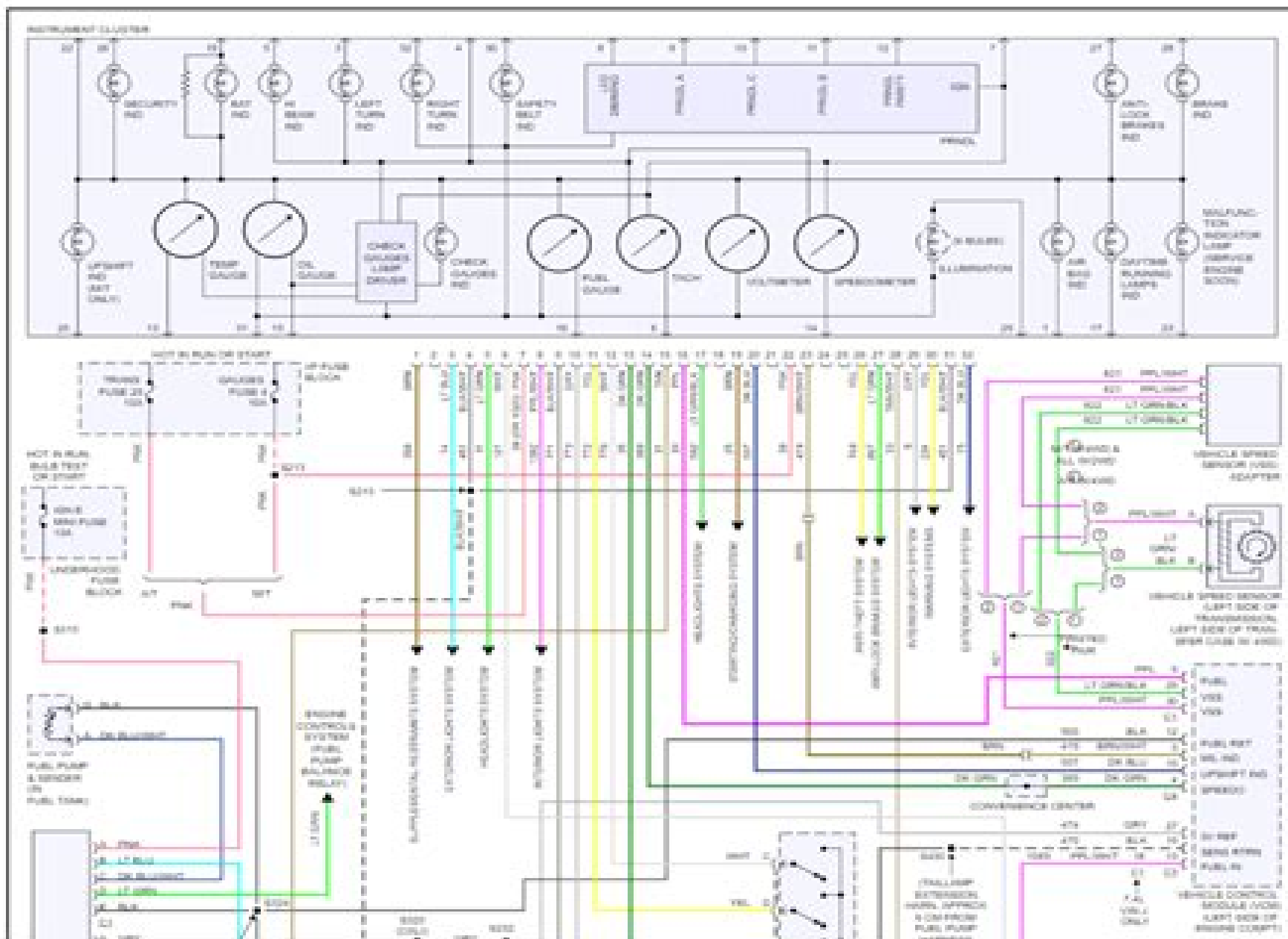
Fig 1: 5.7L VIN R, Instrument Cluster Circuit
