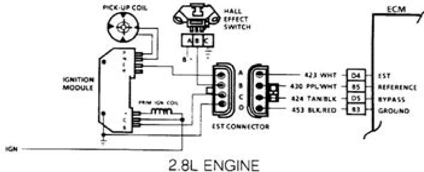
Fig. 45: Code 42, Electronic Spark Timing Schematic
